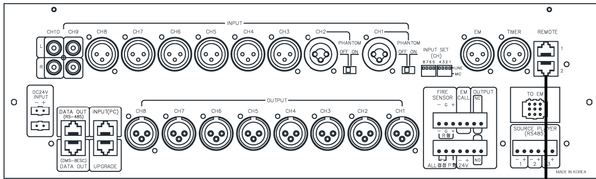
DMS-8MC(Main Controller)
